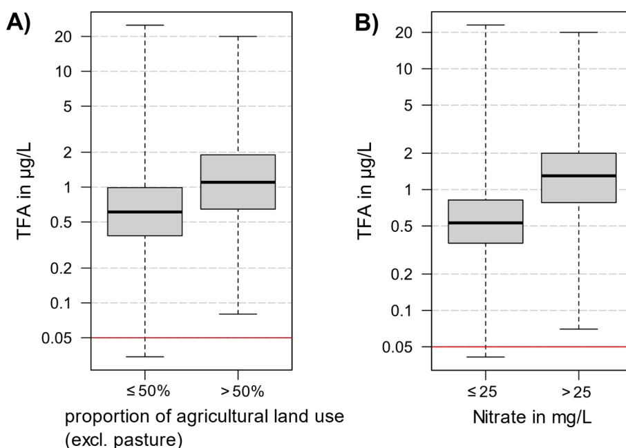
Fig. 5. A) Censored boxplots of the TFA concentration grouped by proportion of agricultural land use \leq 50 % and > 50 % ( n = 1598 ). B) Censored boxplots of the TFA concentration with data grouped by the nitrate concentration of the samples ( n = 1577 ). Percentiles below the limit of quantification were estimated using regression on order (ROS) statistics. The horizontal red line depicts the LOQ. (For interpretation of the references to colour in this figure legend, the reader is referred to the web version of this article.)
