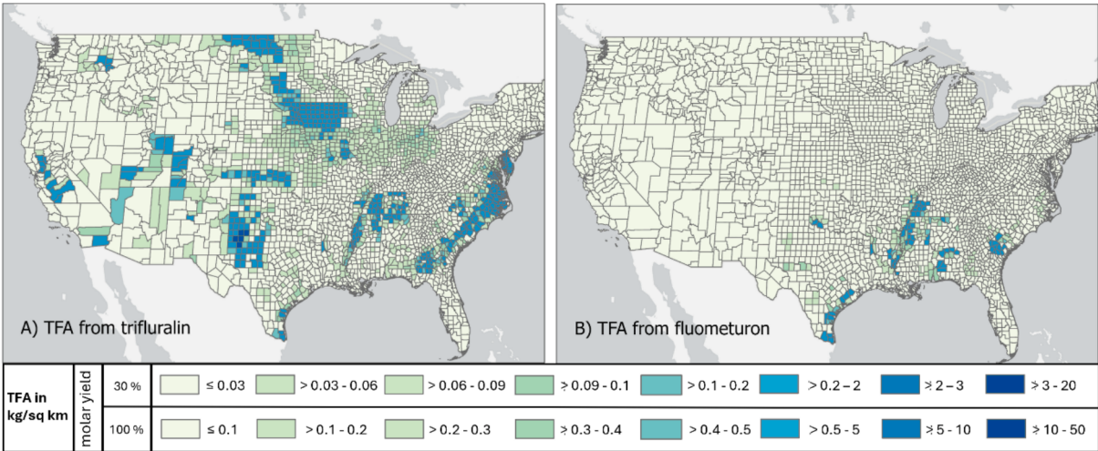
Fig. 4. Relative TFA formation potential in the USA (excluding Hawaii and Alaska) from A) trifluralin and B) fluometuron, based on the estimated amounts applied in each county in 2017 (USGS, 2024), assuming a molar TFA yield of 30 % and 100 %.
