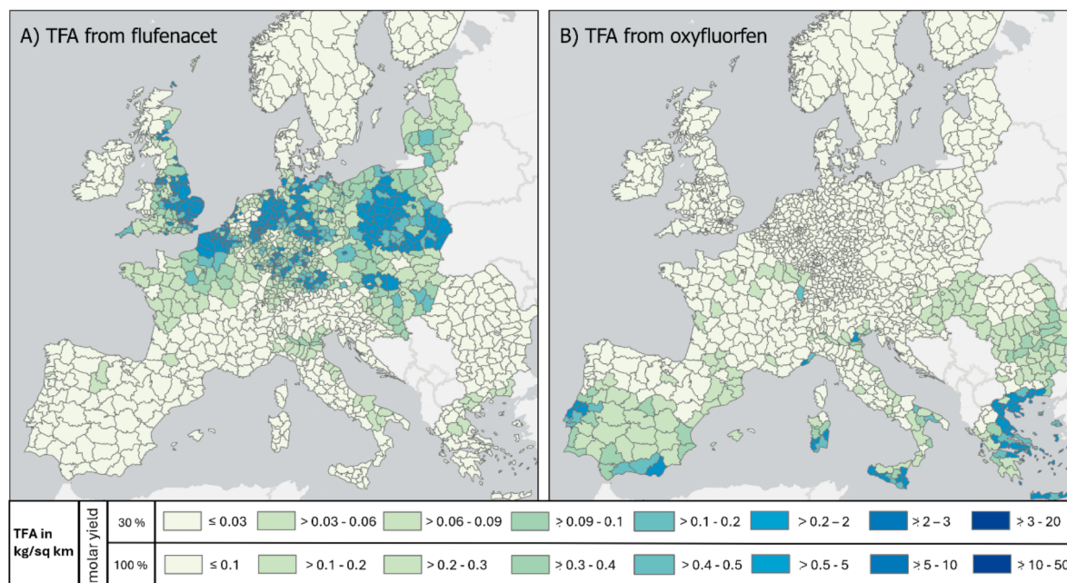
Fig. 2. Relative TFA formation potential in Europe per year from A) flufenacet and B) oxyfluorfen, based on the estimated amounts sold in each NUTS Level 3 region of the EU (Udias et al., 2023) and sales data from Switzerland (2011–2017), a molar TFA yield of 30 % and 100 %.
