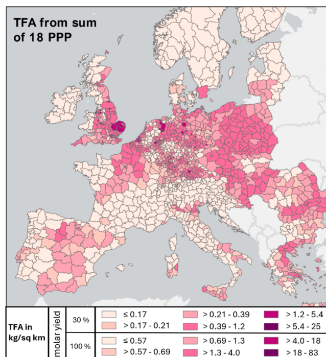
Fig. 1. Total TFA formation potential from PPP in Europe per year, based on the estimated amounts of 18 C-CF 3 -containing PPP sold in each NUTS Level 3 region of the EU between 2011–2017 (Udias et al., 2023) and sales data from Switzerland (2011–2017), assuming a molar TFA yield of 30 % and 100 %.
