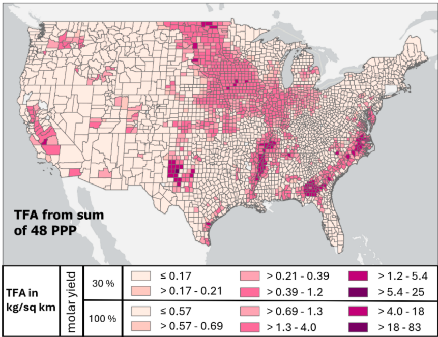
Fig. 3. TFA formation potential from PPP in the continuous USA (excluding Hawaii and Alaska), based on the estimated amounts of 48 C-CF 3 -containing PPP in each county in 2017 (USGS, 2024), assuming a molar TFA yield of 30 % and 100 %.
